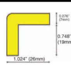
Corner Guard Type E
