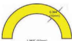
Pipe Guard Type R50
