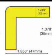
Corner Guard Type H
