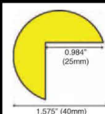
Corner Guard Type A
