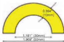
Pipe Guard Type R30
